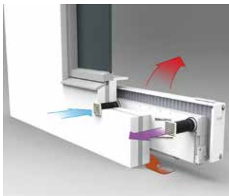
Principe werking Climarad in radiator versie
